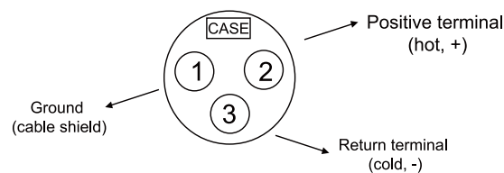
XLR Terminal (male) Pins on BDP-105 D
