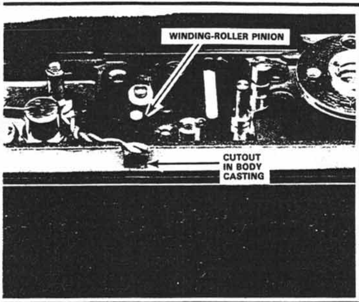
Figure 155 Shutter released
