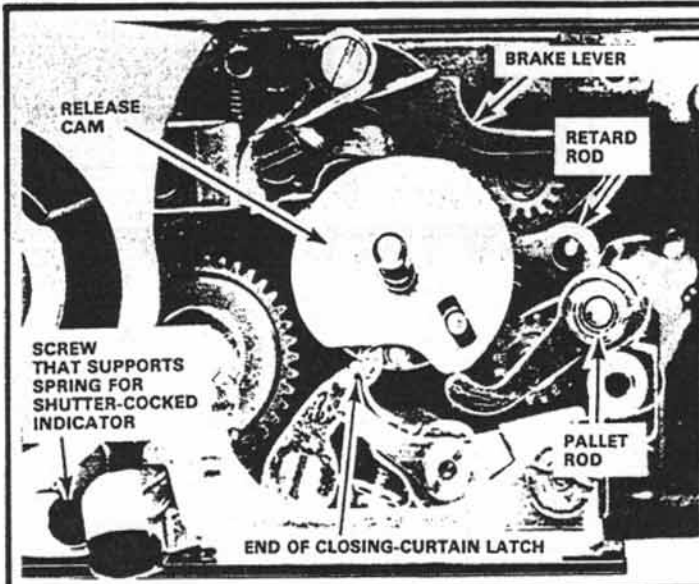
Figure 206 Shutter cocked
