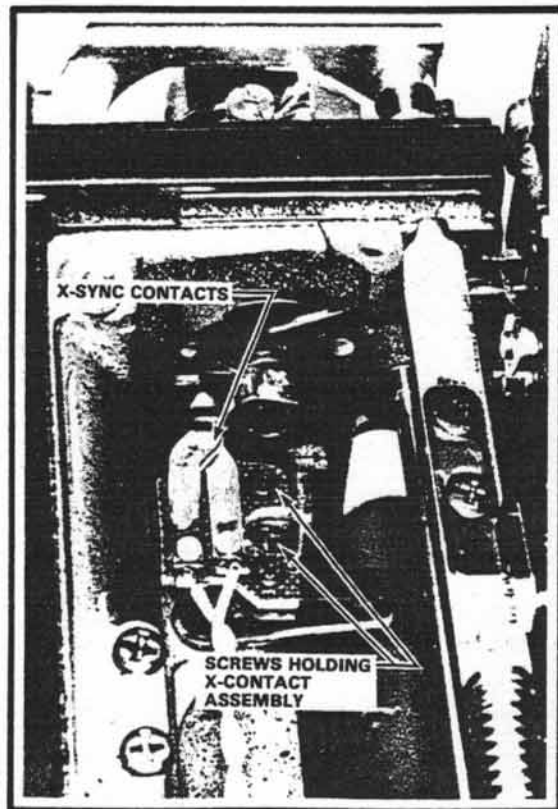
Figure 82 Shutter Released
