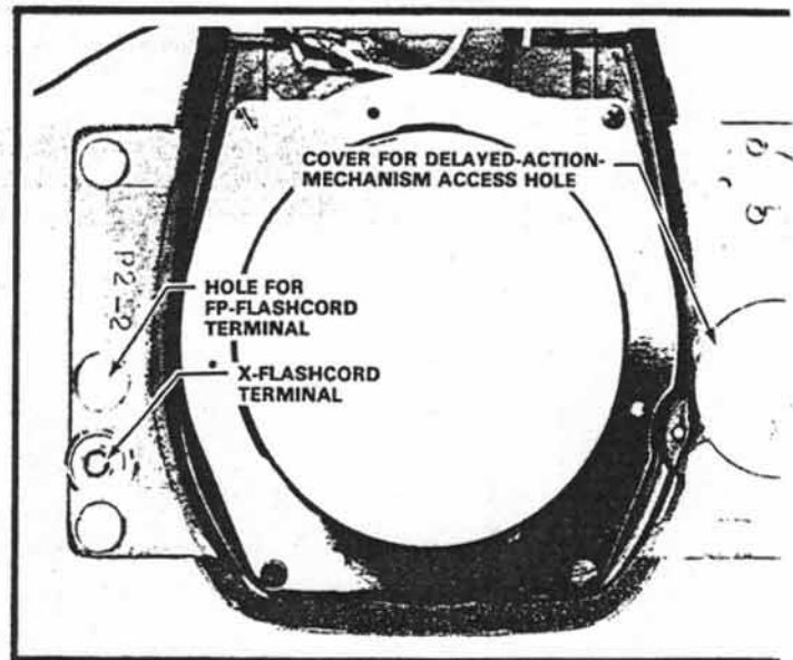
Figure 86 Back of front standard
