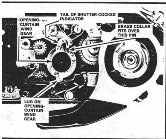
Figure 121 Shutter released
