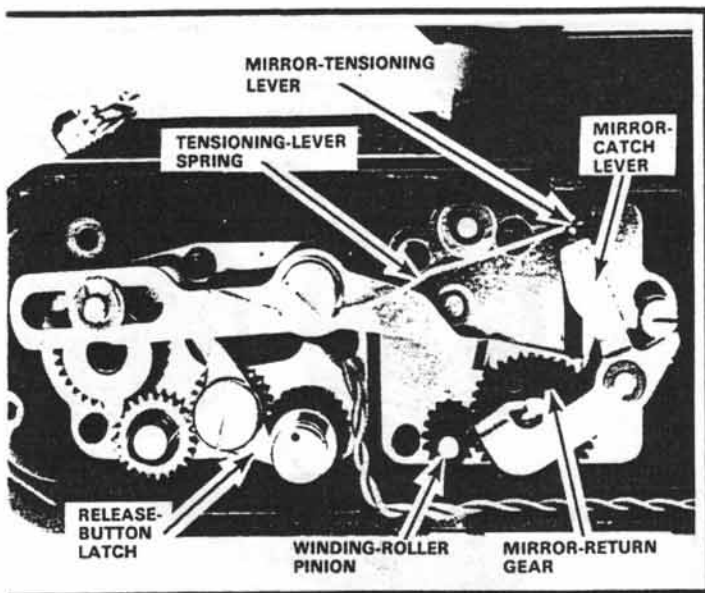
Figure 12 Shutter cocked
