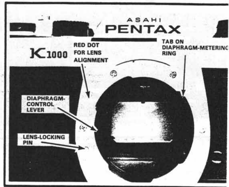
Figure 6 The lens-locking pin drops into a slot in the back of the lens (Fig. 7). Pushing in the lens latch withdraws the lens-locking pin; you can then remove the lens.
