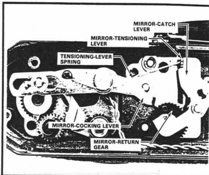
Figure 88 Shutter cocked
