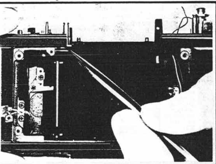
Figure 189 Release the shutter by disengaging the opening-curtain latch.
