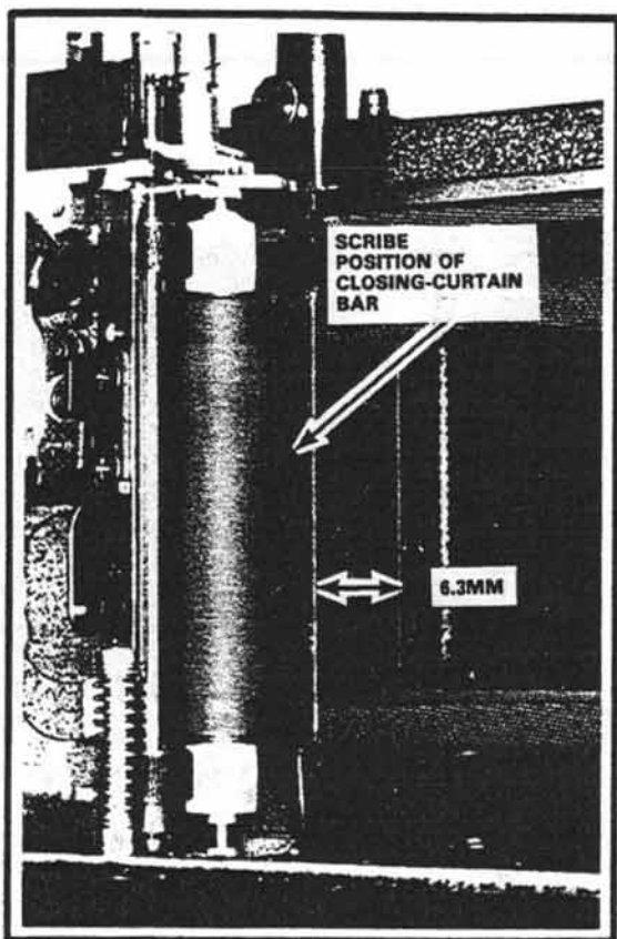
Figure 152 Shutter held open by closing-curtain latch.
