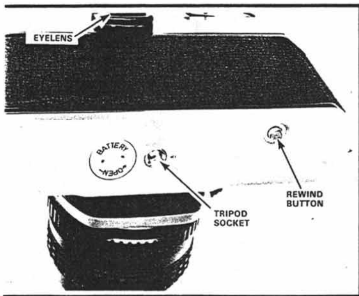
Figure 4 The K1000 uses one 1.5V silver-oxide battery (Eveready S-76 or equivalent)
