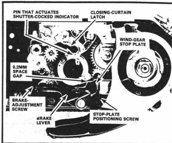
Figure 122 Shutter cocked
