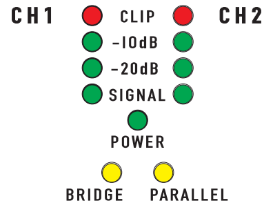
Two-Channel Models
