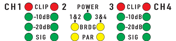
Four-Channel Models
