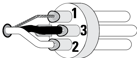
Balanced Inputs XLR Connector
