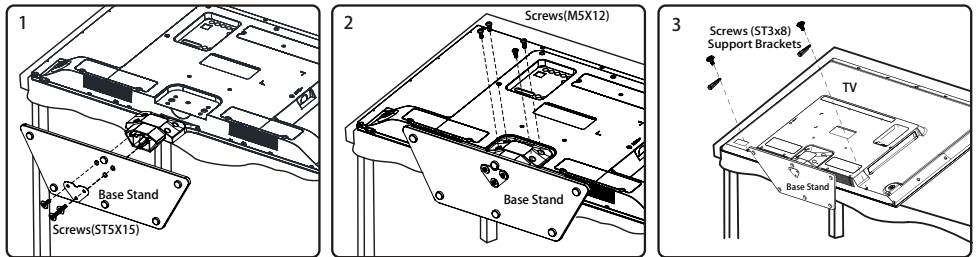
Screws (ST4x15) for models of 32" and 39"
