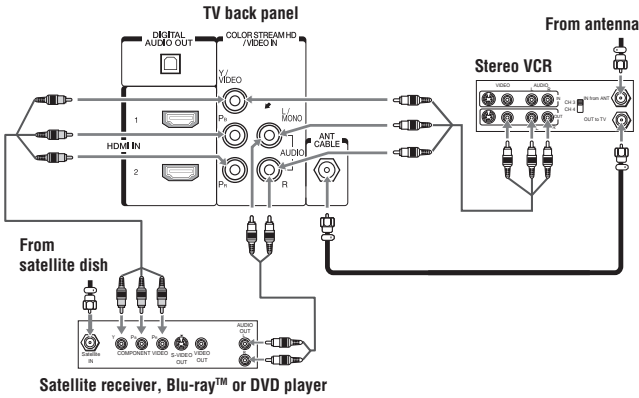
(Sample Illustration) 40/50L3400U—Connecting a Blu-ray™/DVD player or Satellite receiver with Colorstream™ (or VCR).
